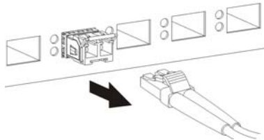
Figure 9 Opening the Transceiver's Latch Example
